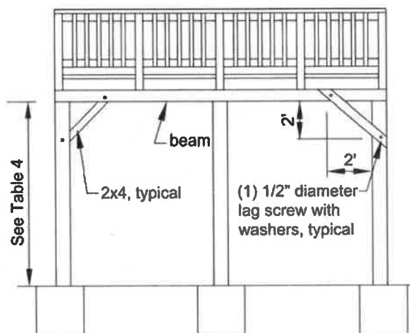
Figure 10. Diagonal Bracing.
